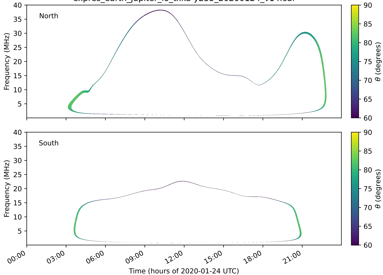
expres_earth_jupiter_io_txka-y235_20200124_v14.cdf
