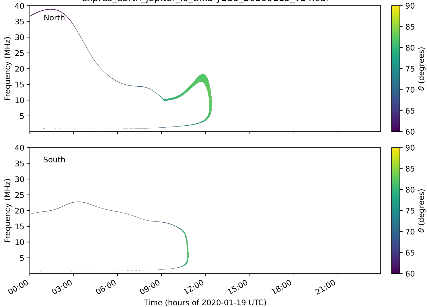
expres_earth_jupiter_io_txka-y235_20200119_v14.cdf
