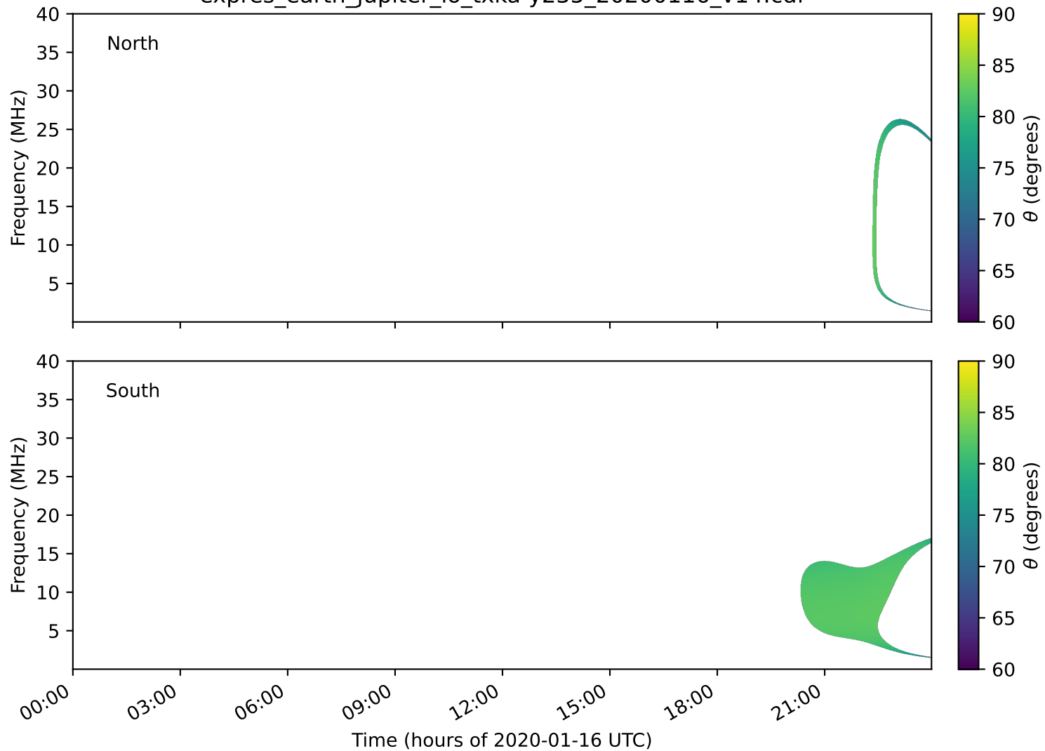
expres_earth_jupiter_io_txka-y235_20200116_v14.cdf
