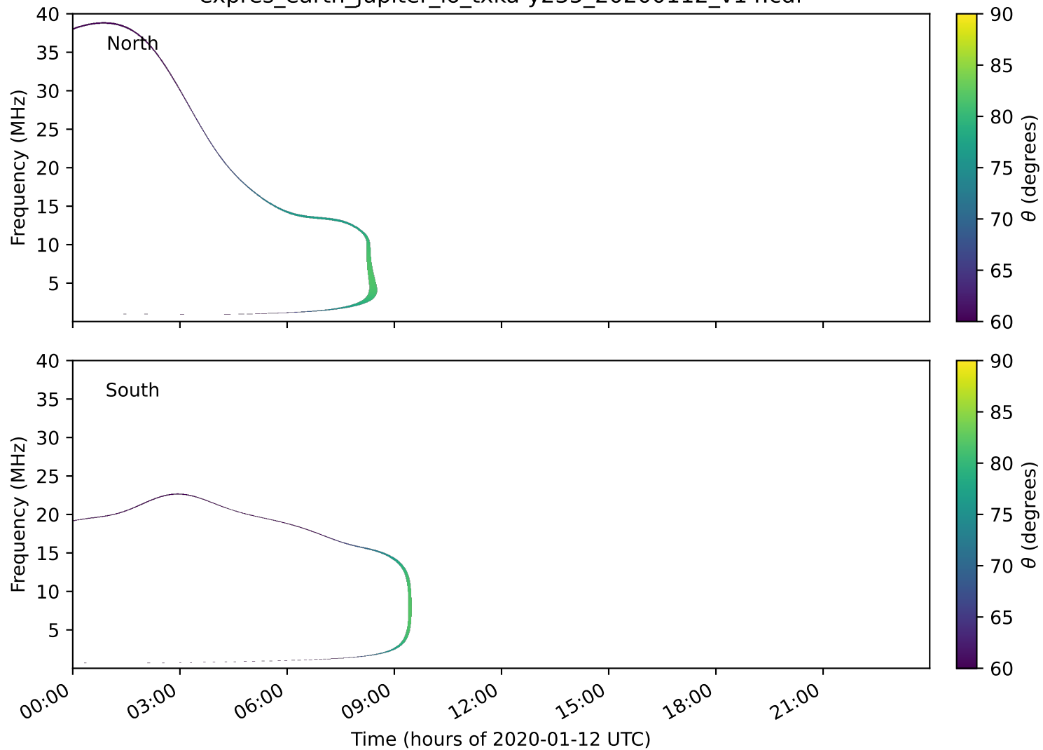
expres_earth_jupiter_io_txka-y235_20200112_v14.cdf
