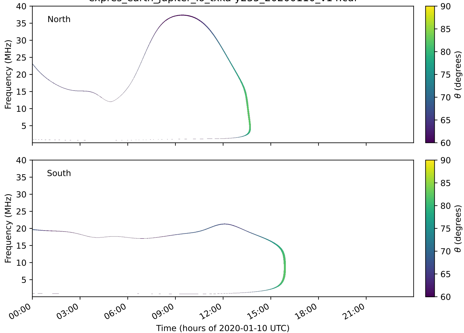
expres_earth_jupiter_io_txka-y235_20200110_v14.cdf
