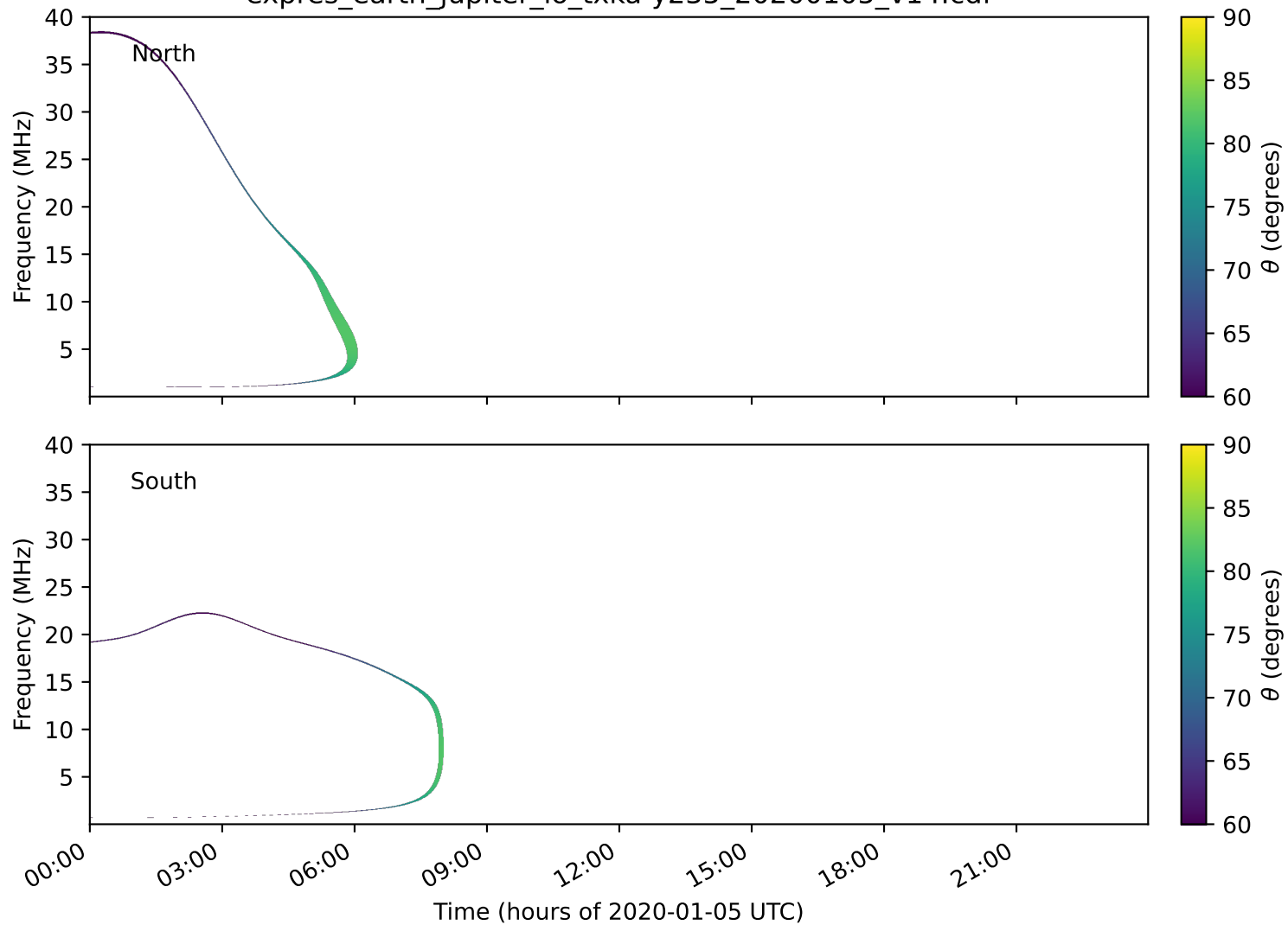
expres_earth_jupiter_io_txka-y235_20200105_v14.cdf
