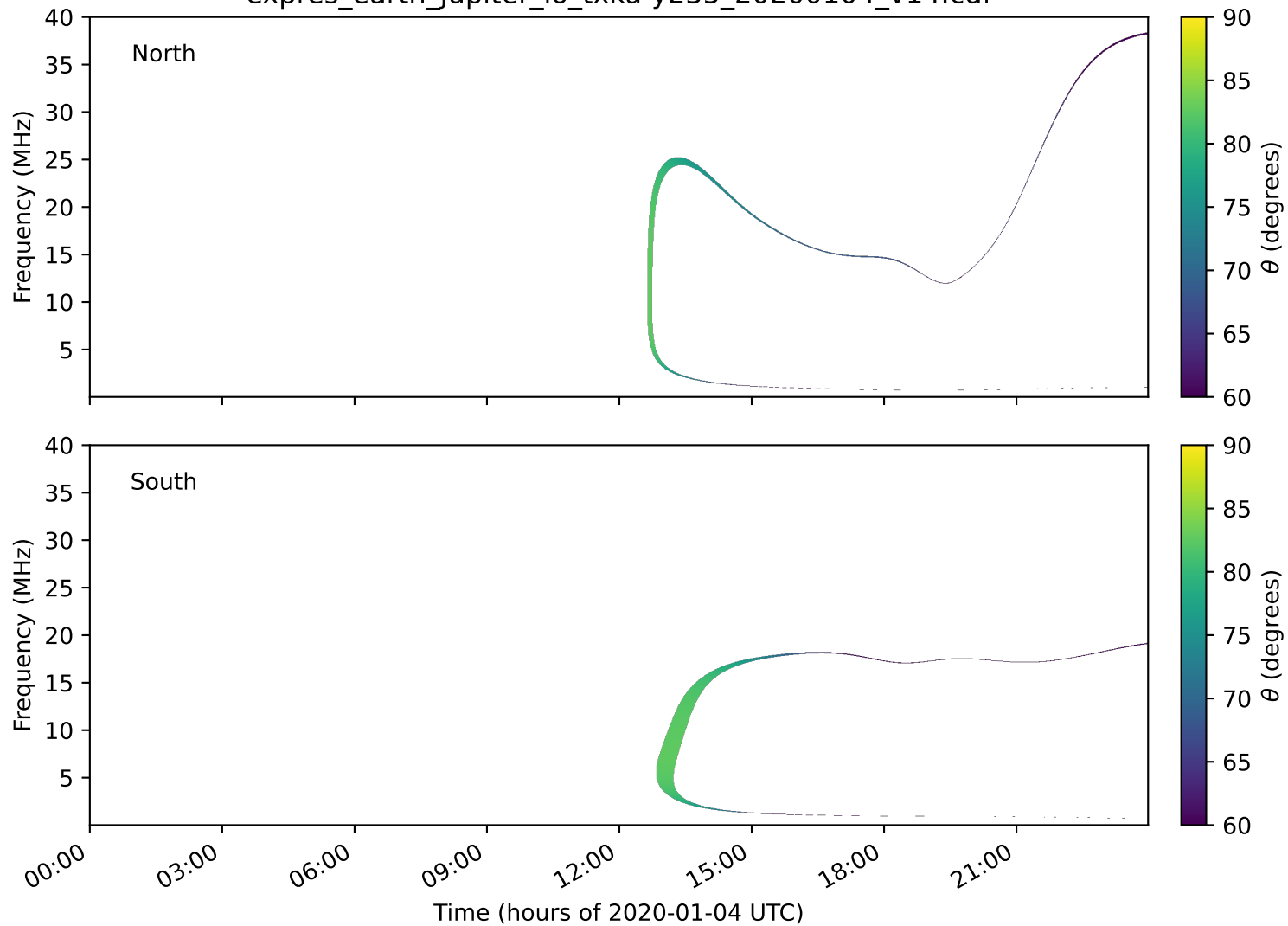
expres_earth_jupiter_io_txka-y235_20200104_v14.cdf
