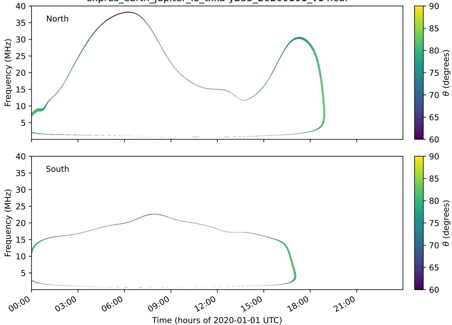
expres_earth_jupiter_io_txka-y235_20200101_v14.cdf
