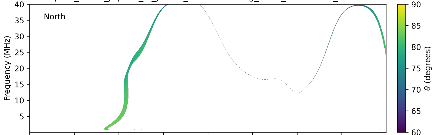
expres_earth_jupiter_io_jrm33_lossc-wid1deg_3kev_20200131_v11.cdf
