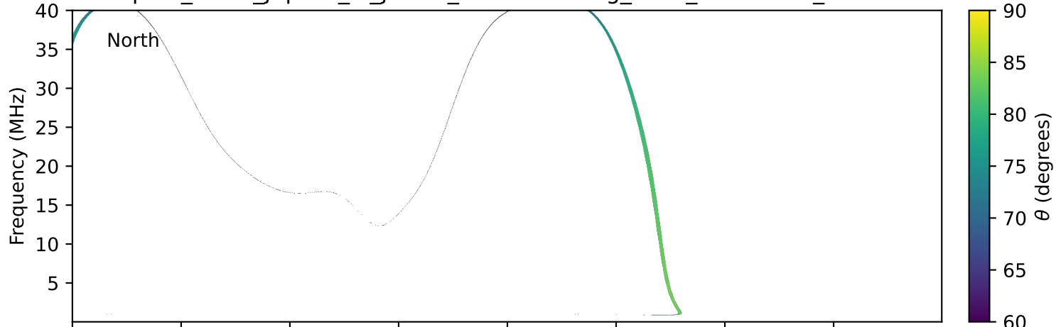
expres_earth_jupiter_io_jrm33_lossc-wid1deg_3kev_20200126_v11.cdf
