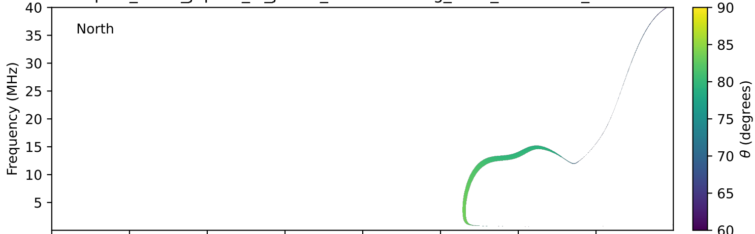
expres_earth_jupiter_io_jrm33_lossc-wid1deg_3kev_20200118_v11.cdf
