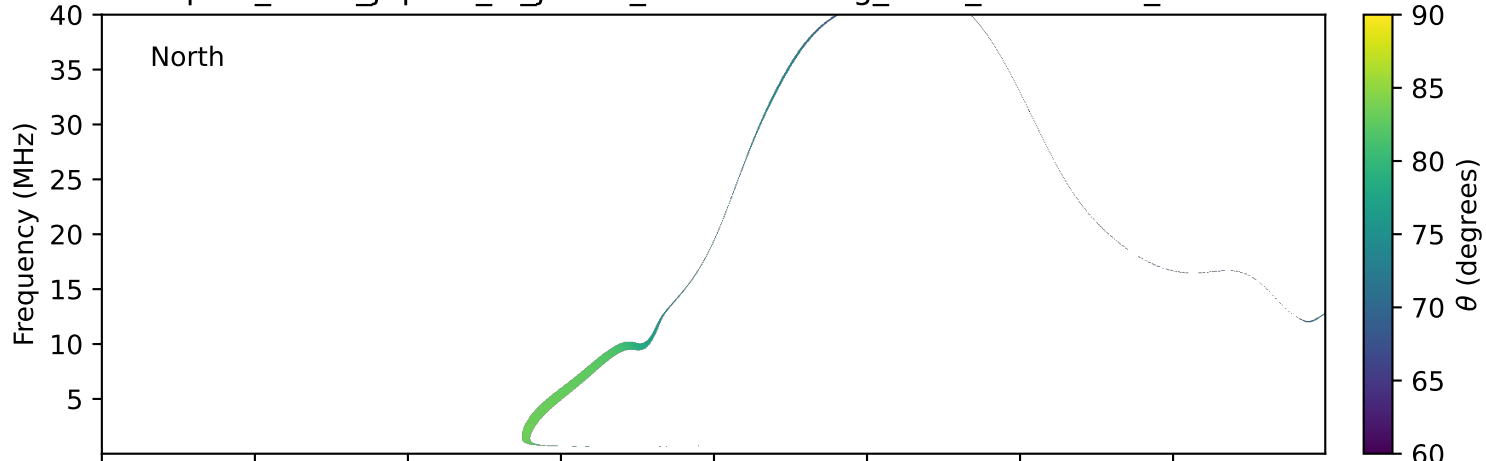
expres_earth_jupiter_io_jrm33_lossc-wid1deg_3kev_20200113_v11.cdf
