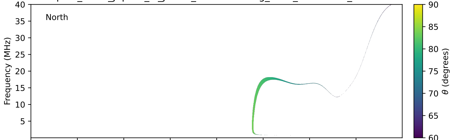
expres_earth_jupiter_io_jrm33_lossc-wid1deg_3kev_20200111_v11.cdf
