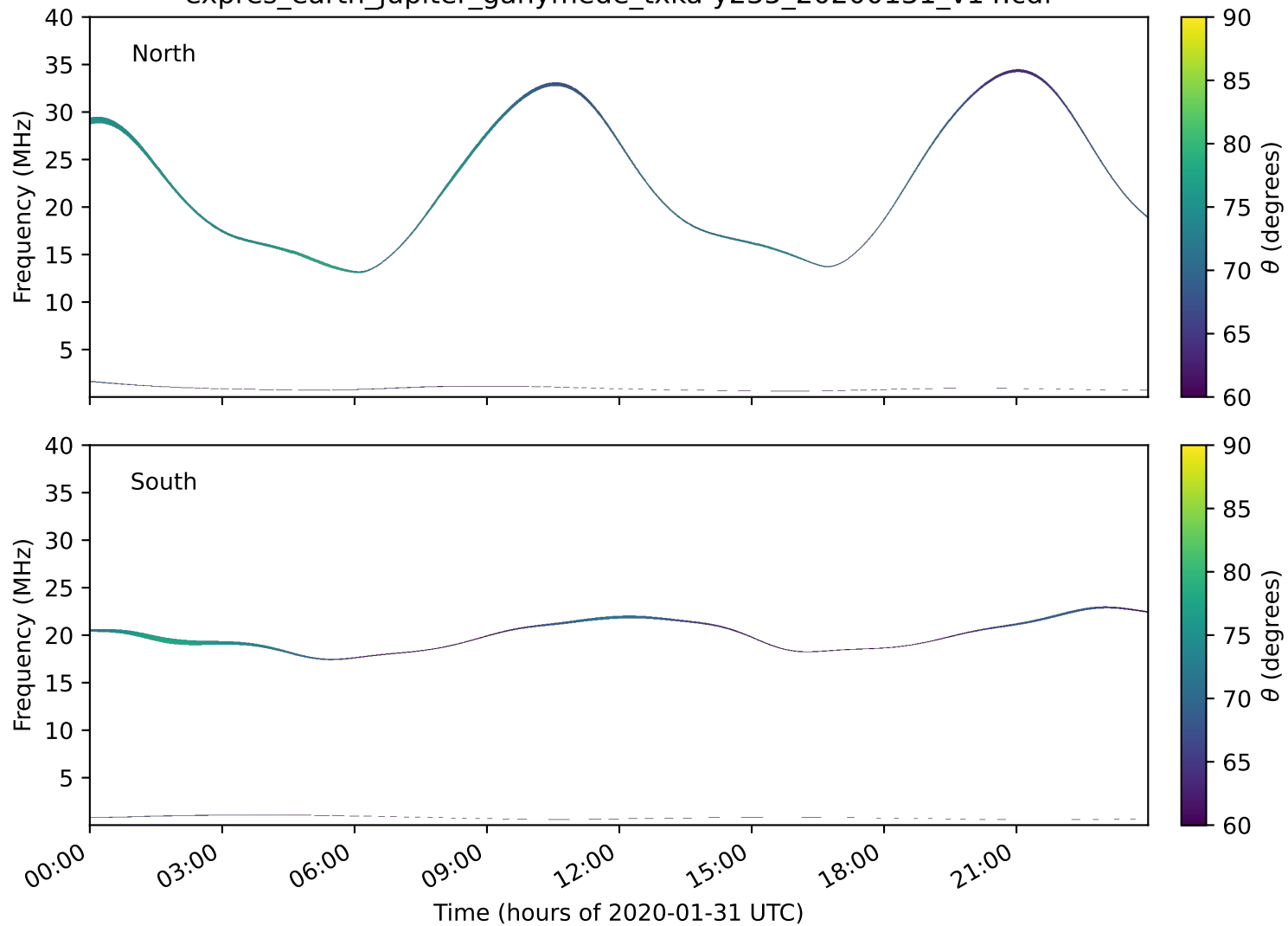
expres_earth_jupiter_ganymede_txka-y235_20200131_v14.cdf
