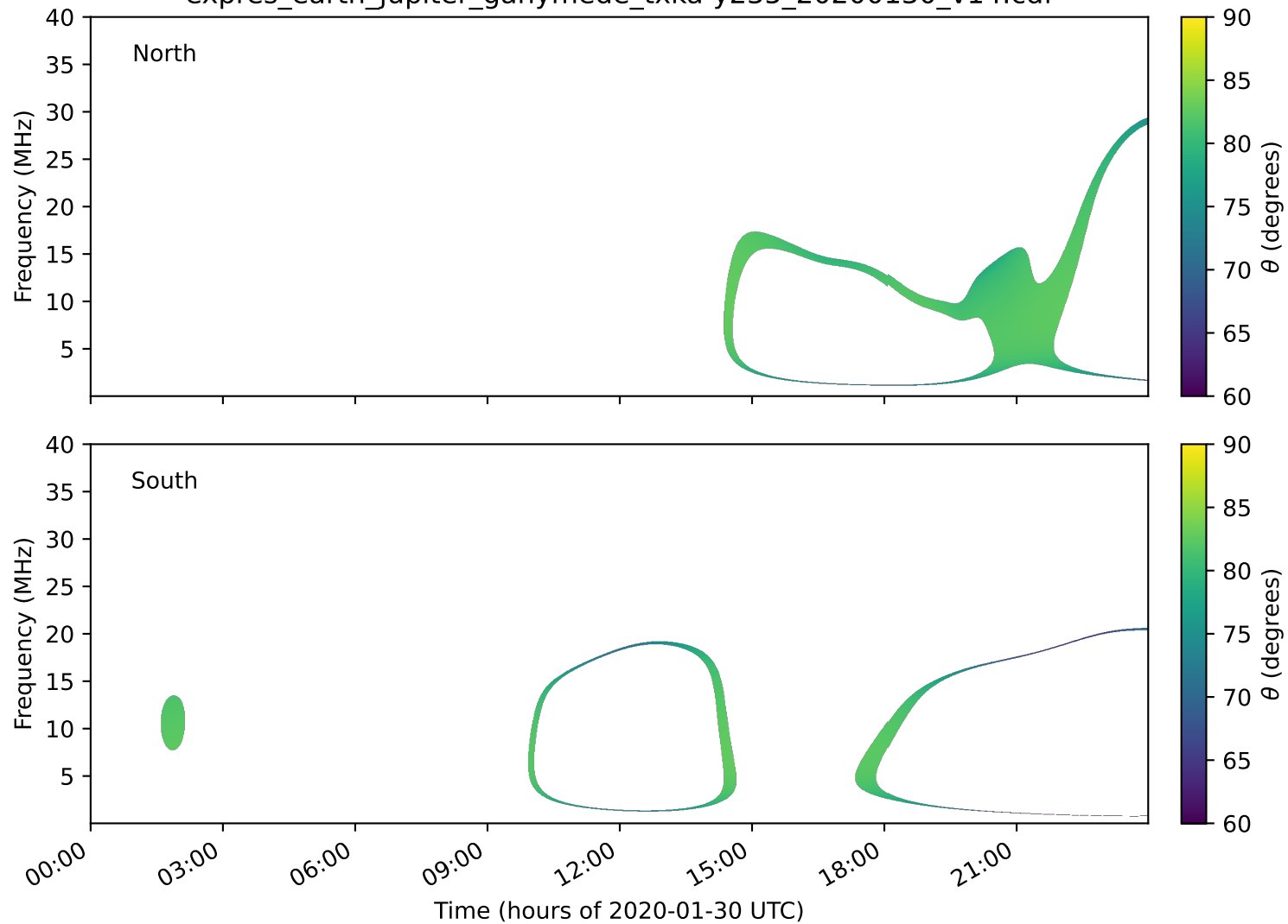
expres_earth_jupiter_ganymede_txka-y235_20200130_v14.cdf
