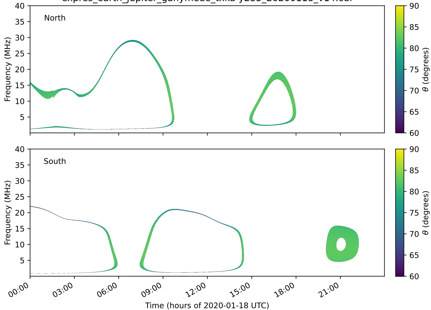
expres_earth_jupiter_ganymede_txka-y235_20200118_v14.cdf
