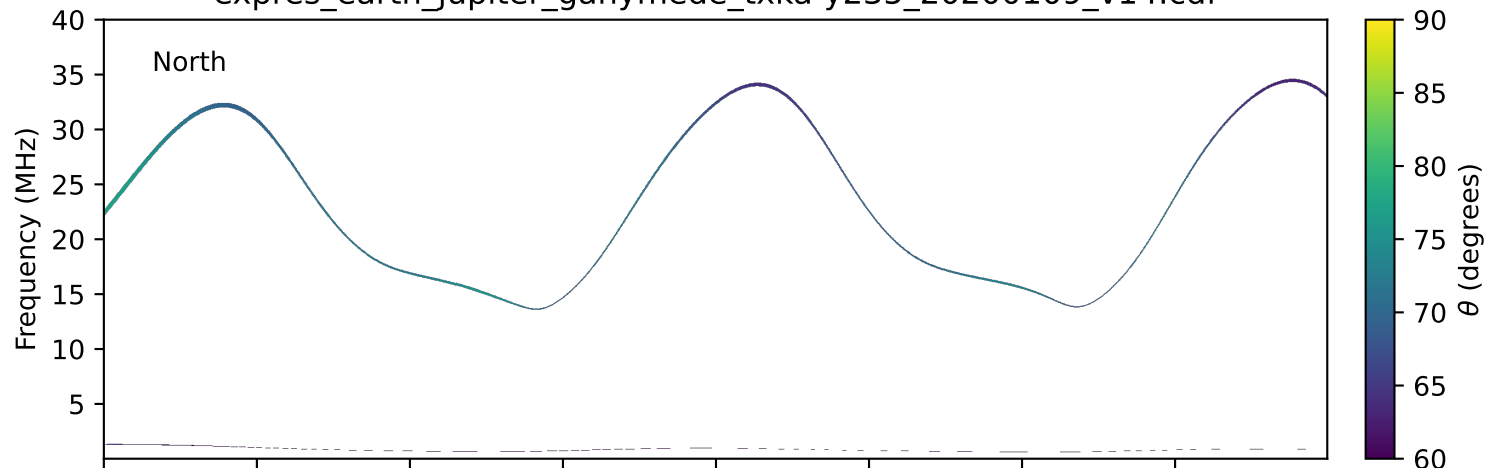
expres_earth_jupiter_ganymede_txka-y235_20200109_v14.cdf
