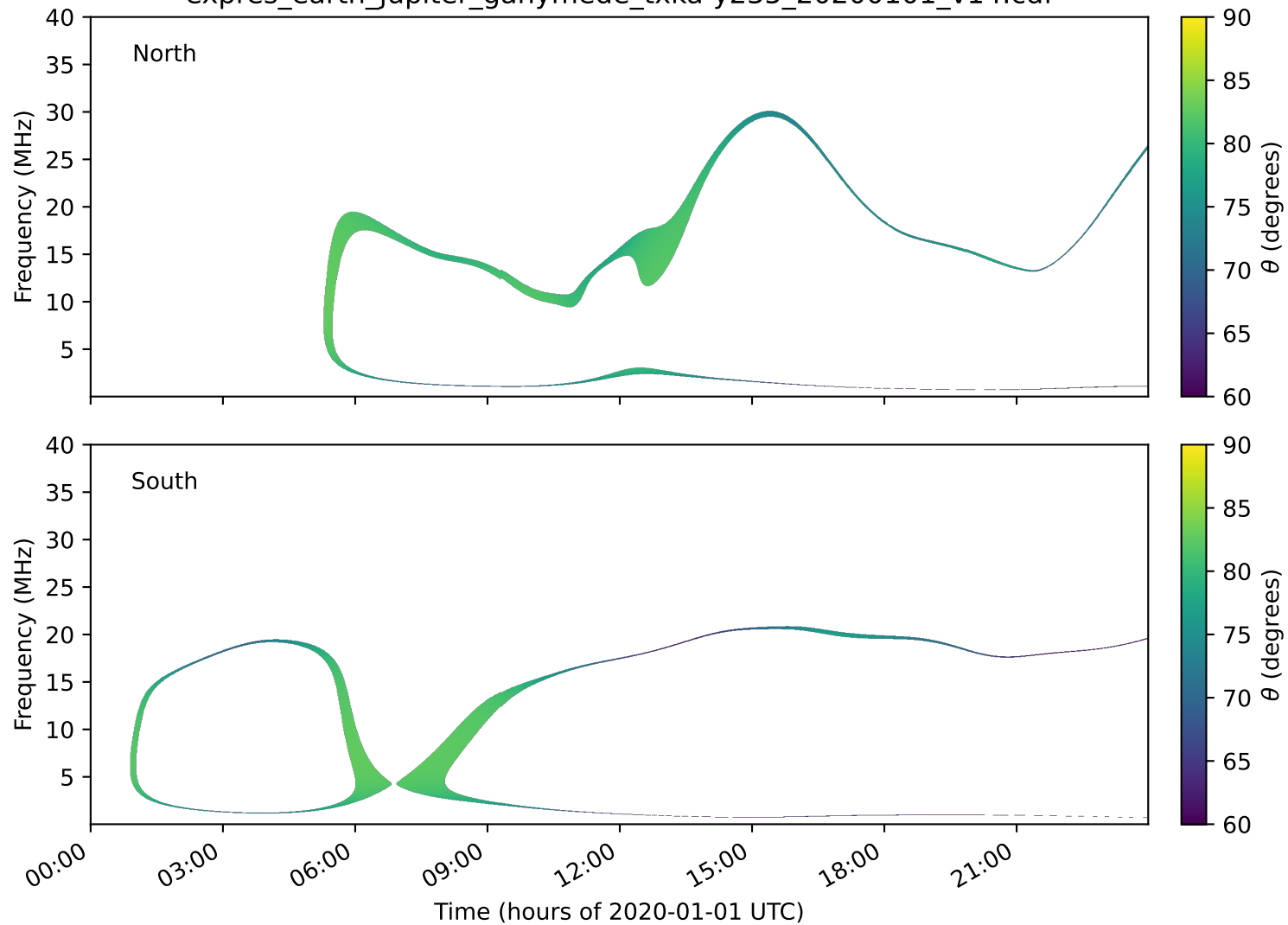
expres_earth_jupiter_ganymede_txka-y235_20200101_v14.cdf
