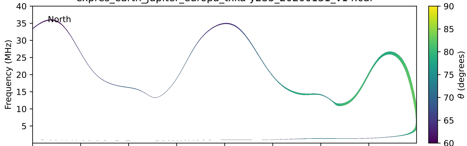
expres_earth_jupiter_europa_txka-y235_20200131_v14.cdf
