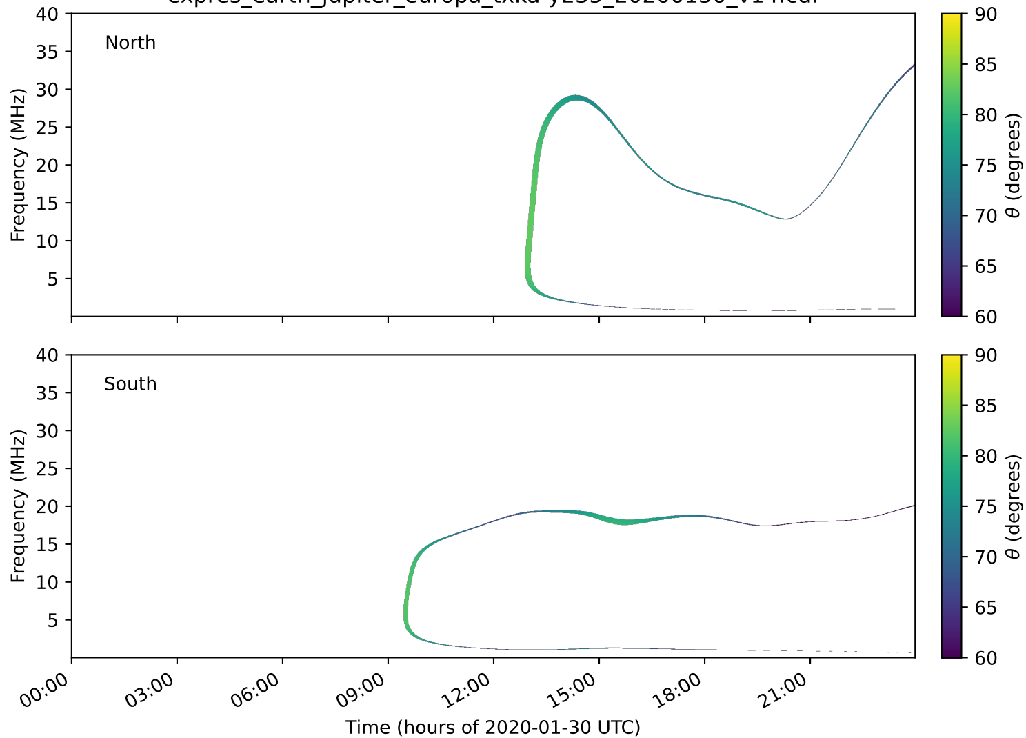
expres_earth_jupiter_europa_txka-y235_20200130_v14.cdf
