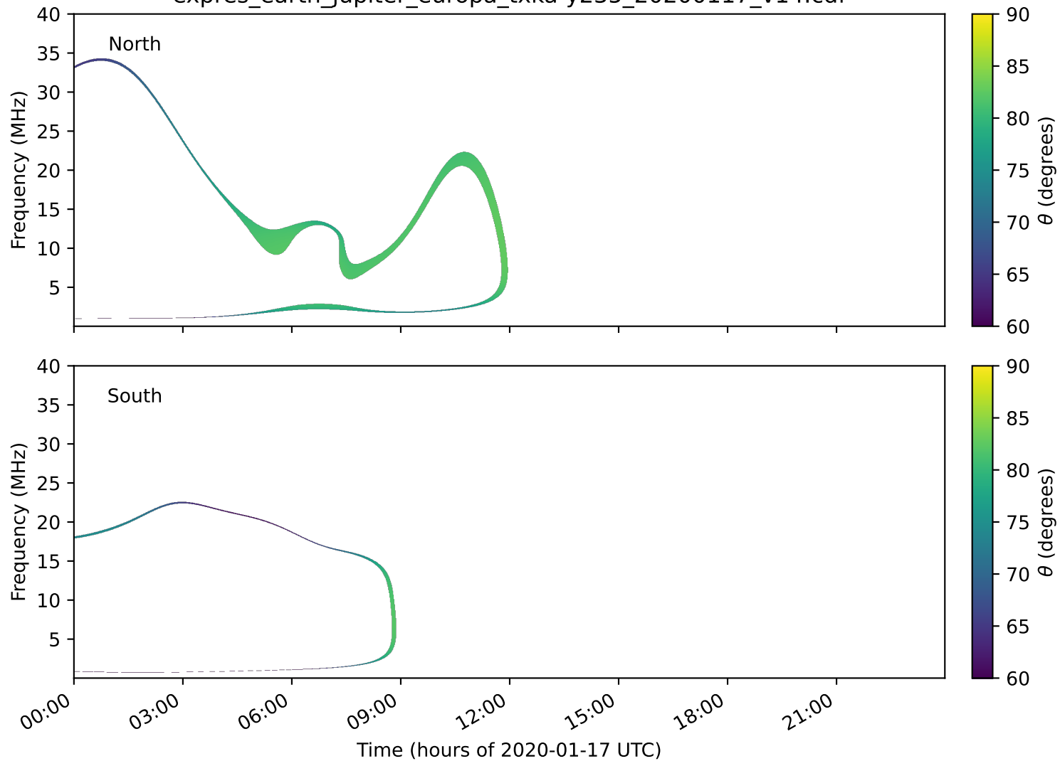
expres_earth_jupiter_europa_txka-y235_20200117_v14.cdf
