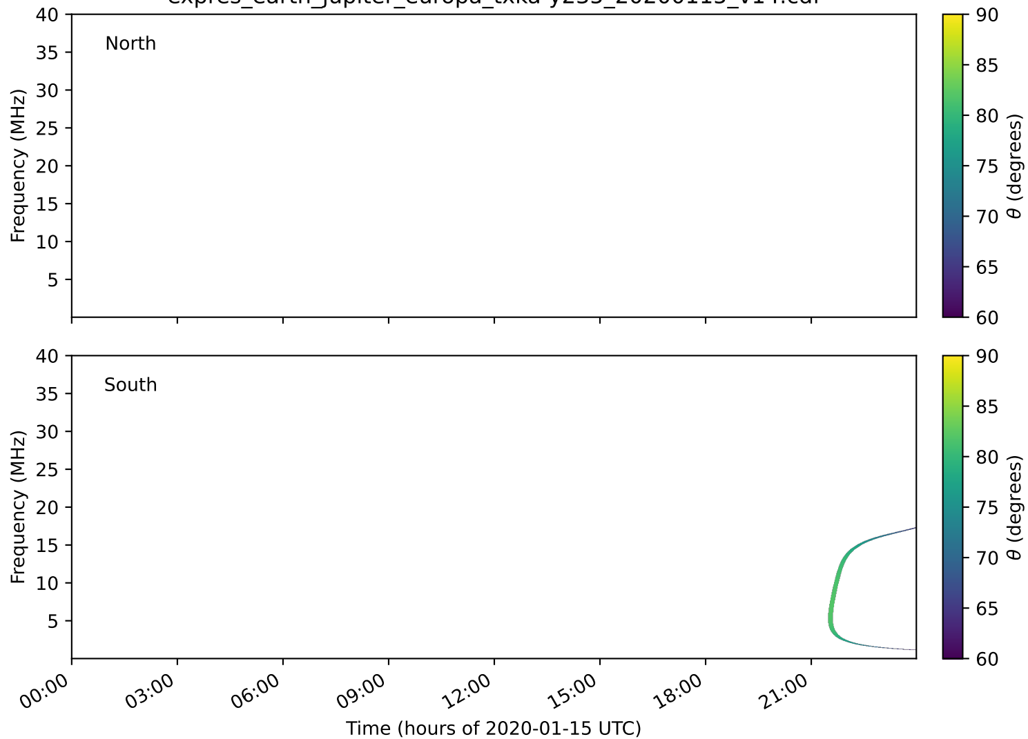
expres_earth_jupiter_europa_txka-y235_20200115_v14.cdf
