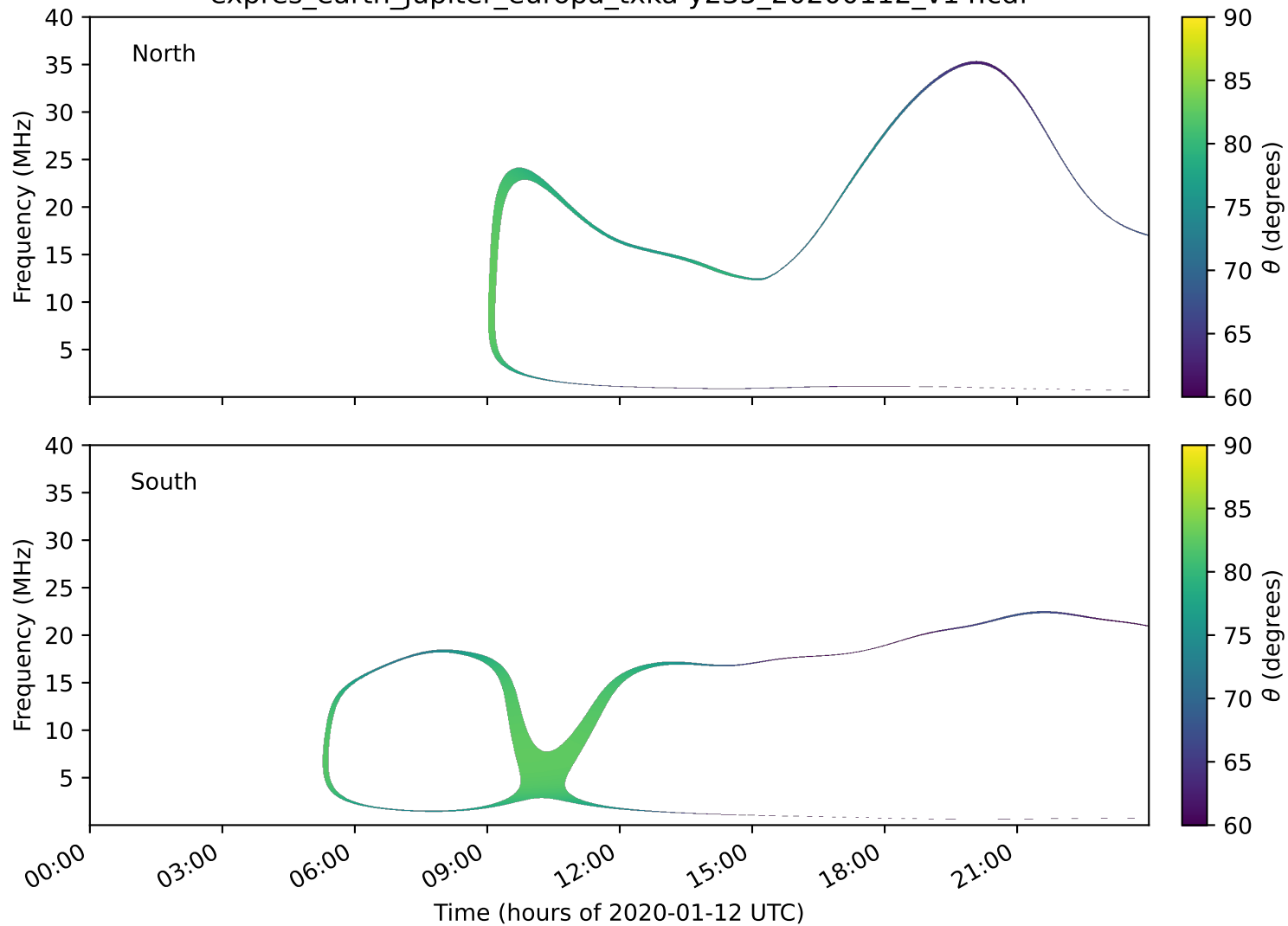
expres_earth_jupiter_europa_txka-y235_20200112_v14.cdf
