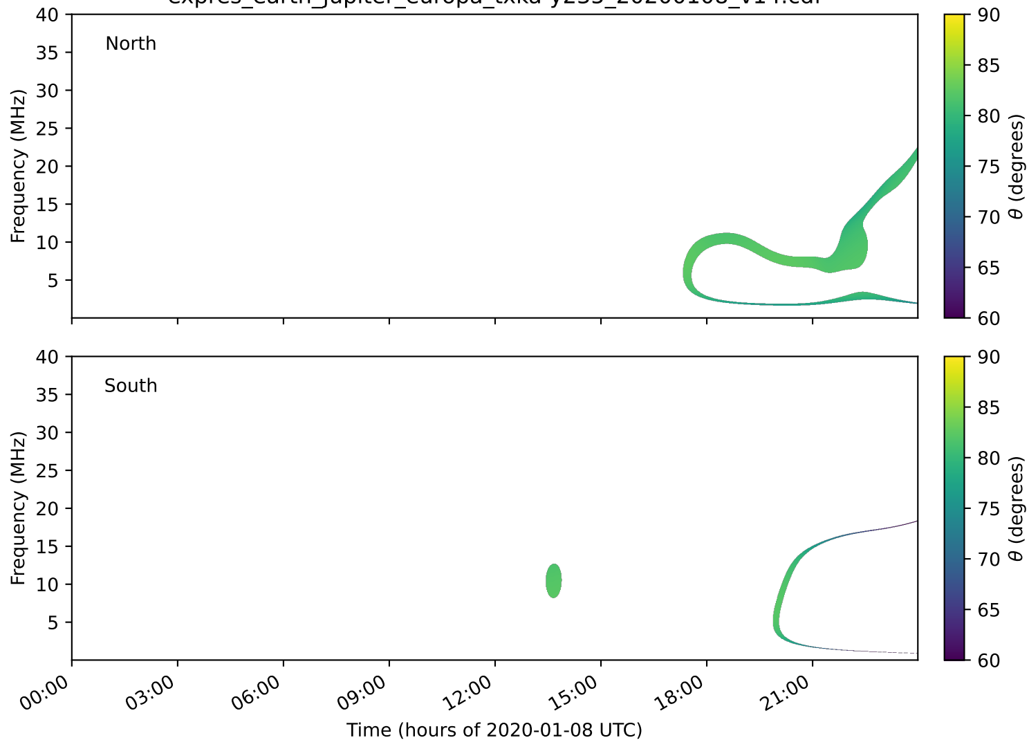
expres_earth_jupiter_europa_txka-y235_20200108_v14.cdf
