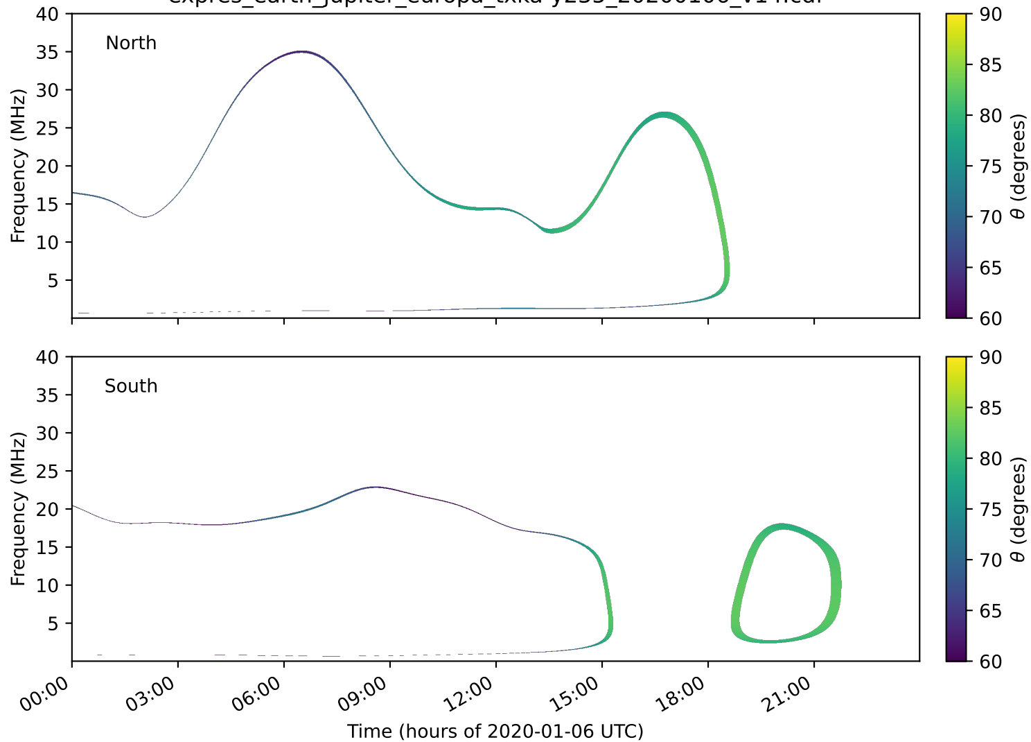
expres_earth_jupiter_europa_txka-y235_20200106_v14.cdf
