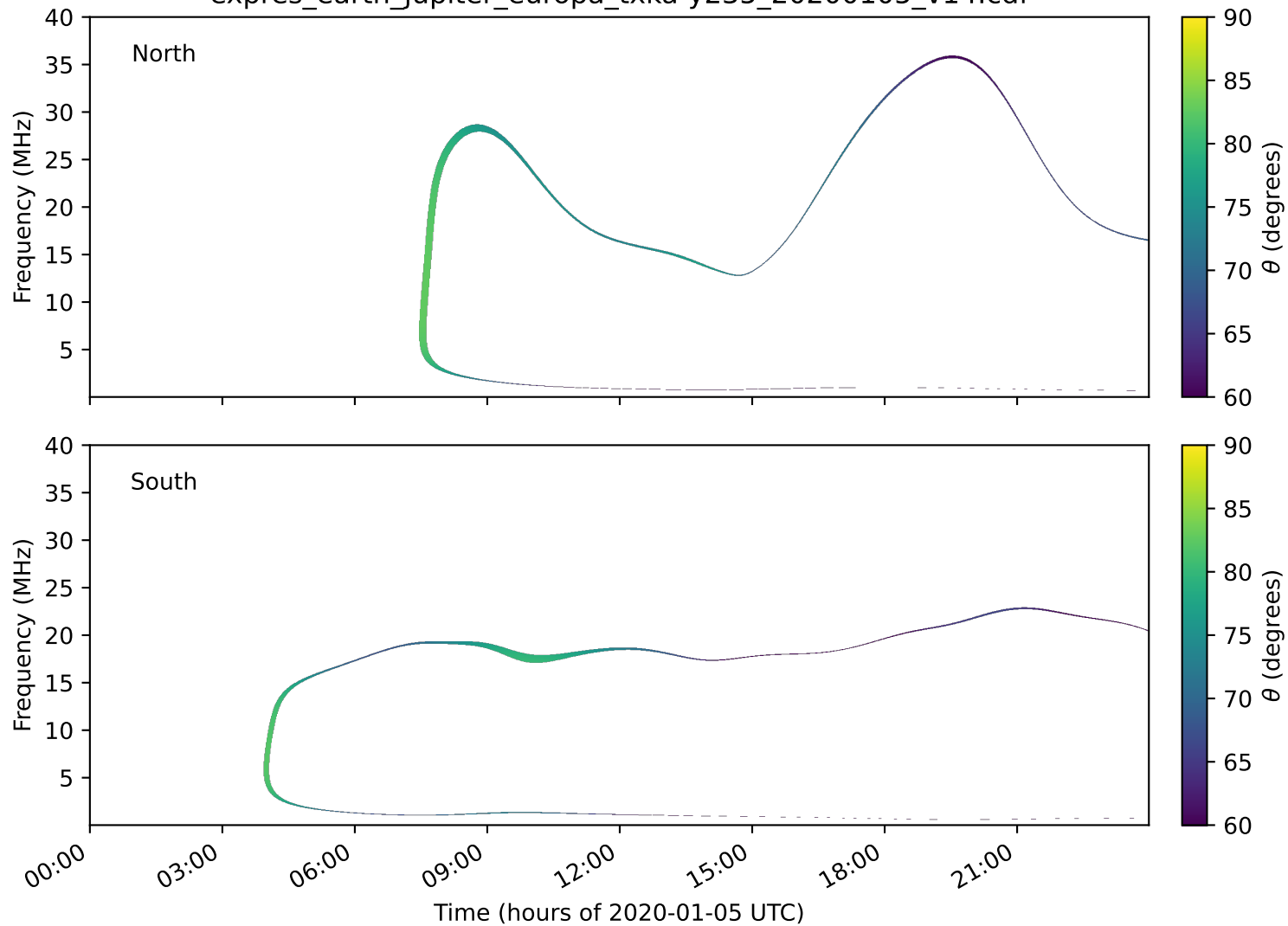
expres_earth_jupiter_europa_txka-y235_20200105_v14.cdf
