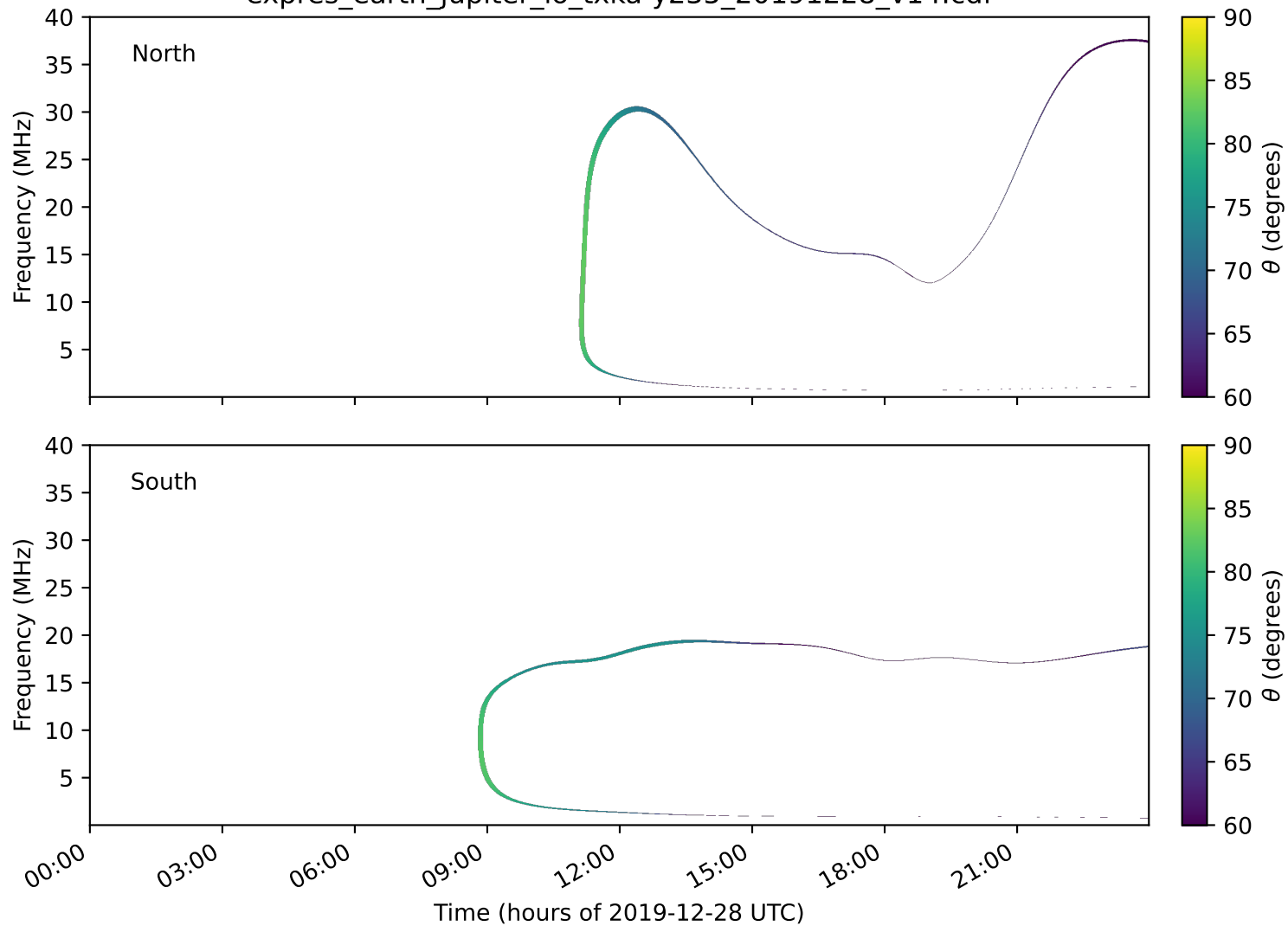
expres_earth_jupiter_io_txka-y235_20191228_v14.cdf
