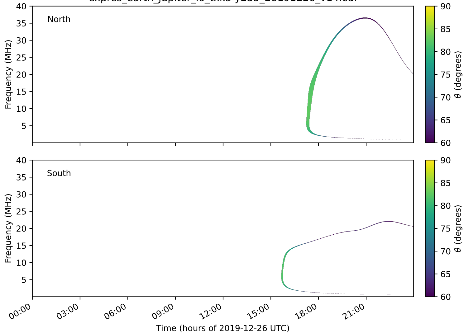
expres_earth_jupiter_io_txka-y235_20191226_v14.cdf
