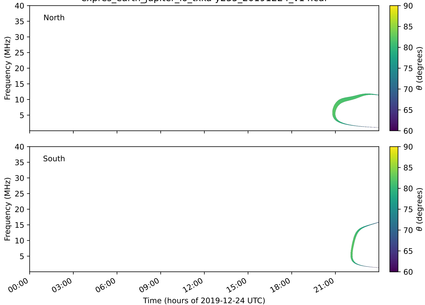
expres_earth_jupiter_io_txka-y235_20191224_v14.cdf
