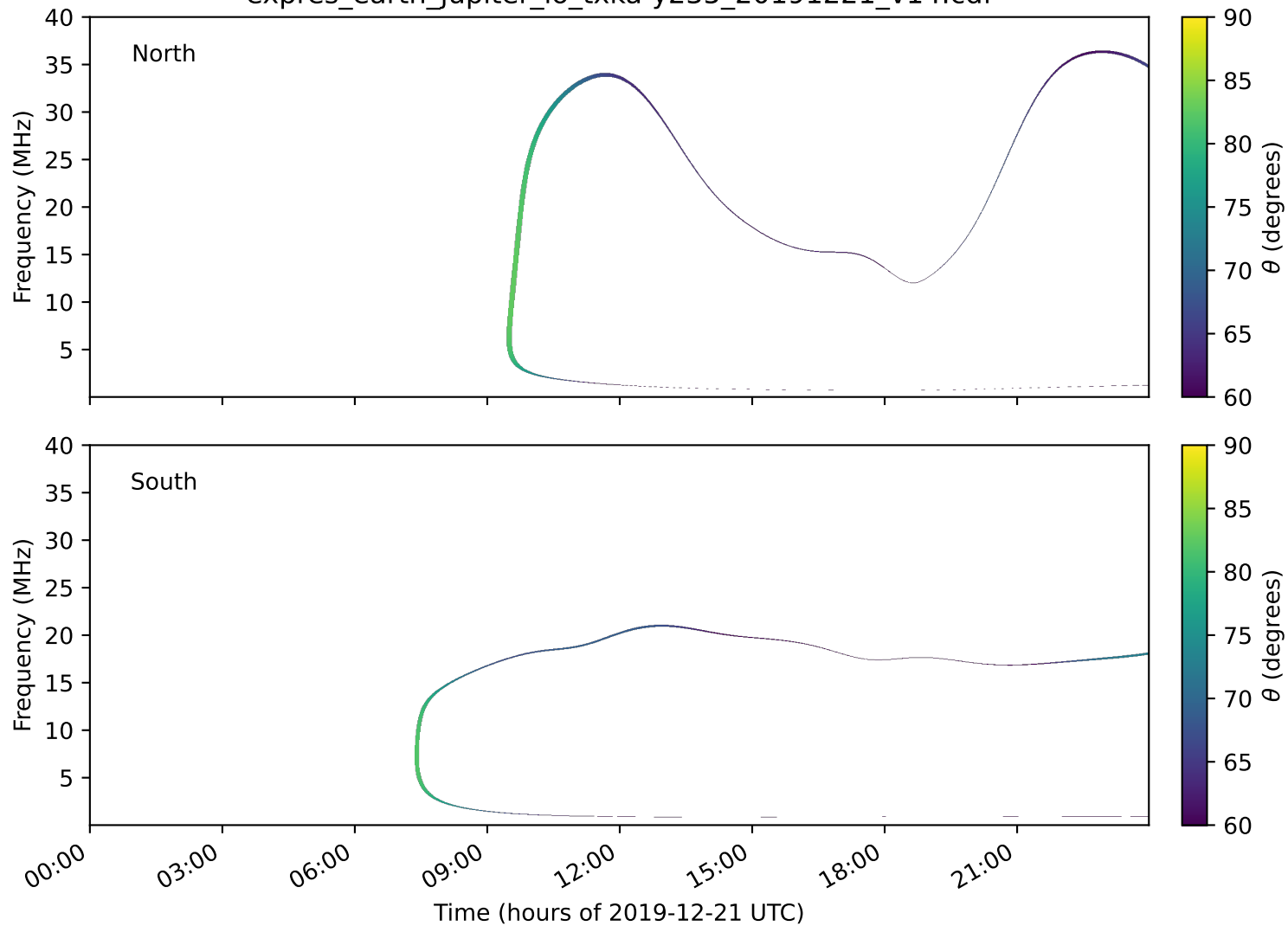
expres_earth_jupiter_io_txka-y235_20191221_v14.cdf
