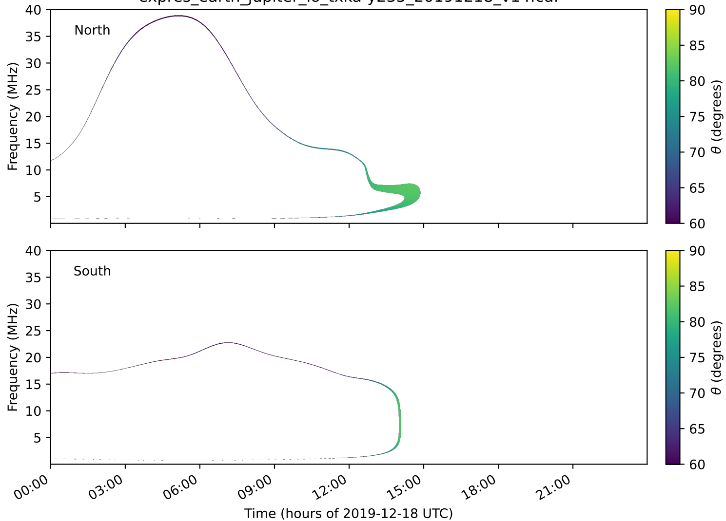
expres_earth_jupiter_io_txka-y235_20191218_v14.cdf
