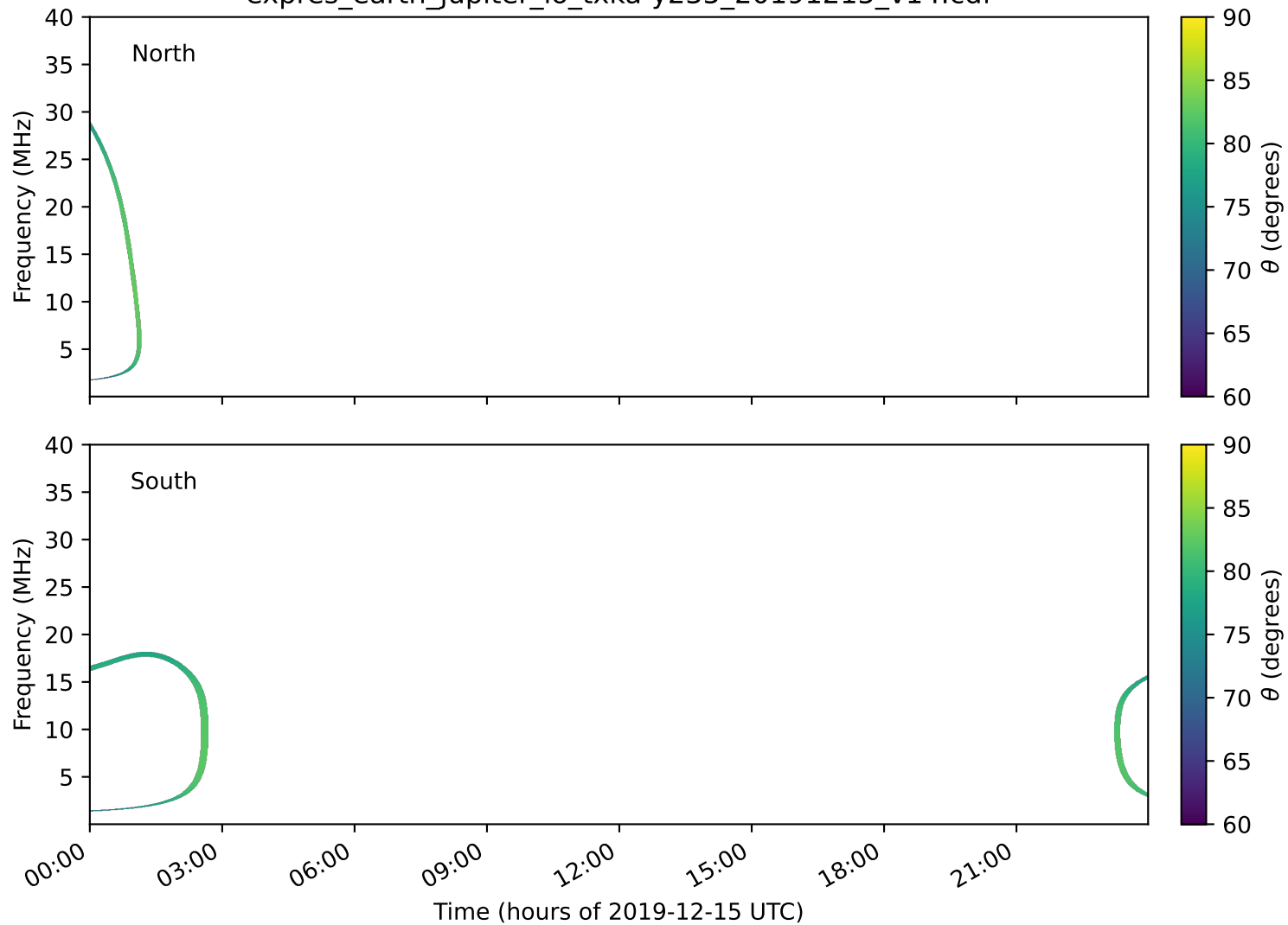
expres_earth_jupiter_io_txka-y235_20191215_v14.cdf
