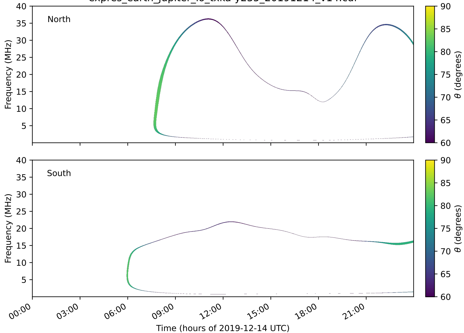
expres_earth_jupiter_io_txka-y235_20191214_v14.cdf
