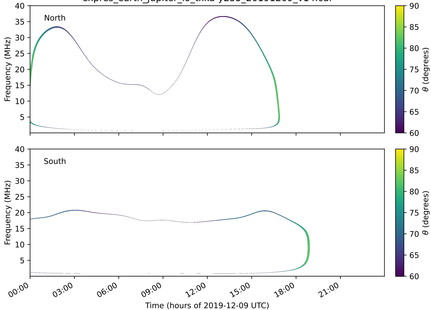
expres_earth_jupiter_io_txka-y235_20191209_v14.cdf
