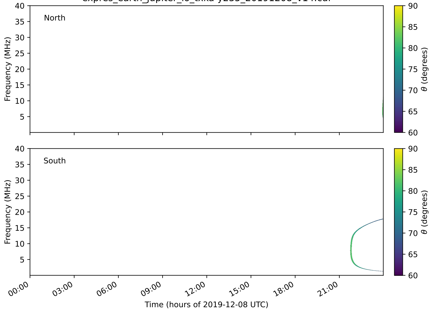
expres_earth_jupiter_io_txka-y235_20191208_v14.cdf
