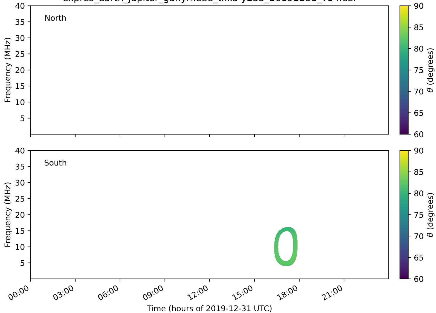
expres_earth_jupiter_ganymede_txka-y235_20191231_v14.cdf
