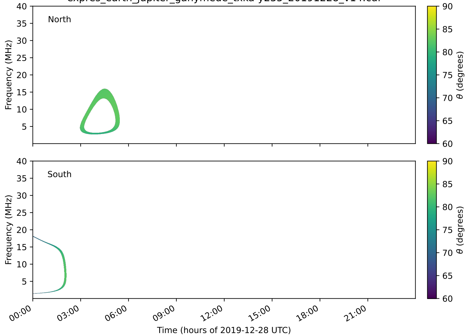
expres_earth_jupiter_ganymede_txka-y235_20191228_v14.cdf
