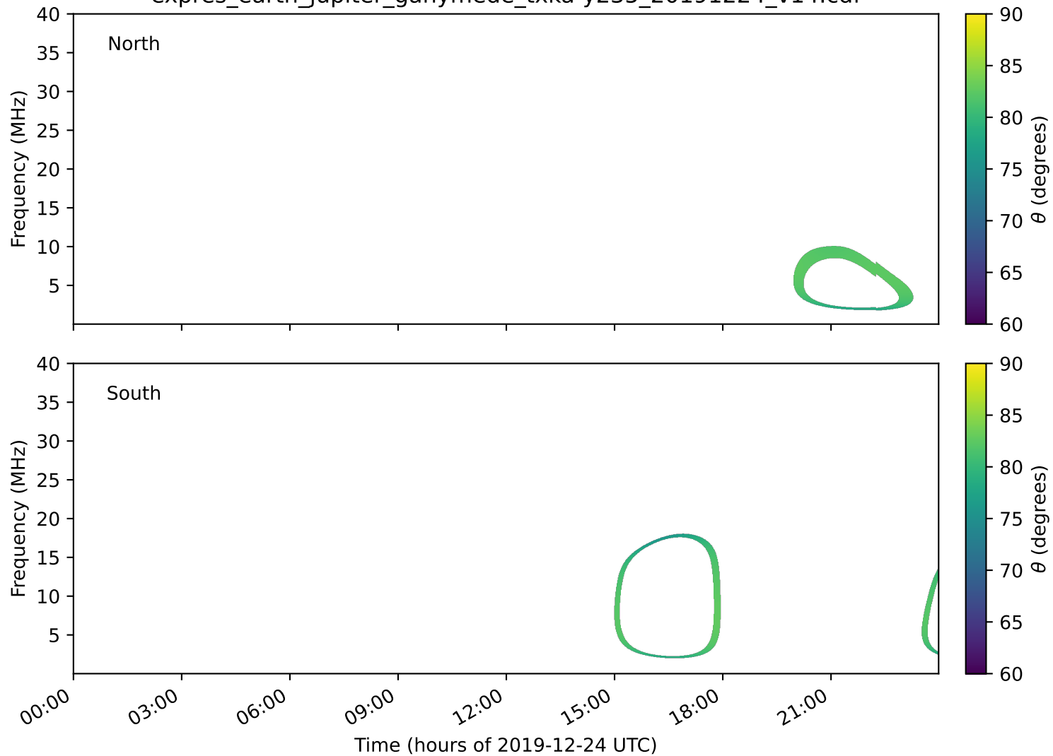
expres_earth_jupiter_ganymede_txka-y235_20191224_v14.cdf
