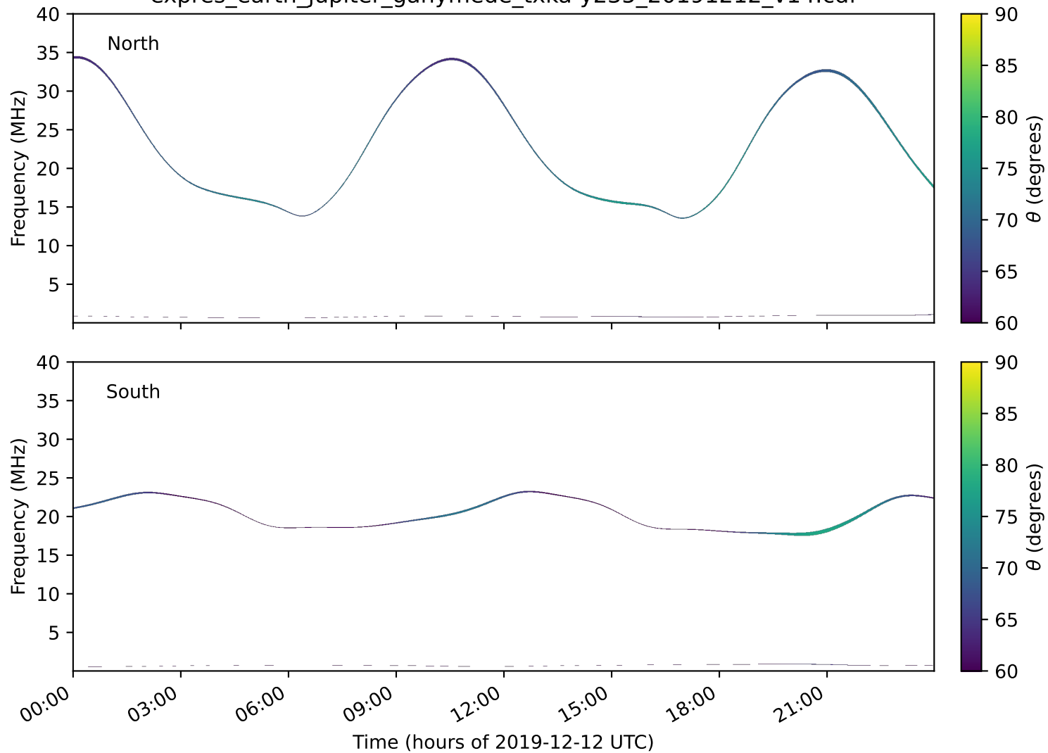
expres_earth_jupiter_ganymede_txka-y235_20191212_v14.cdf
