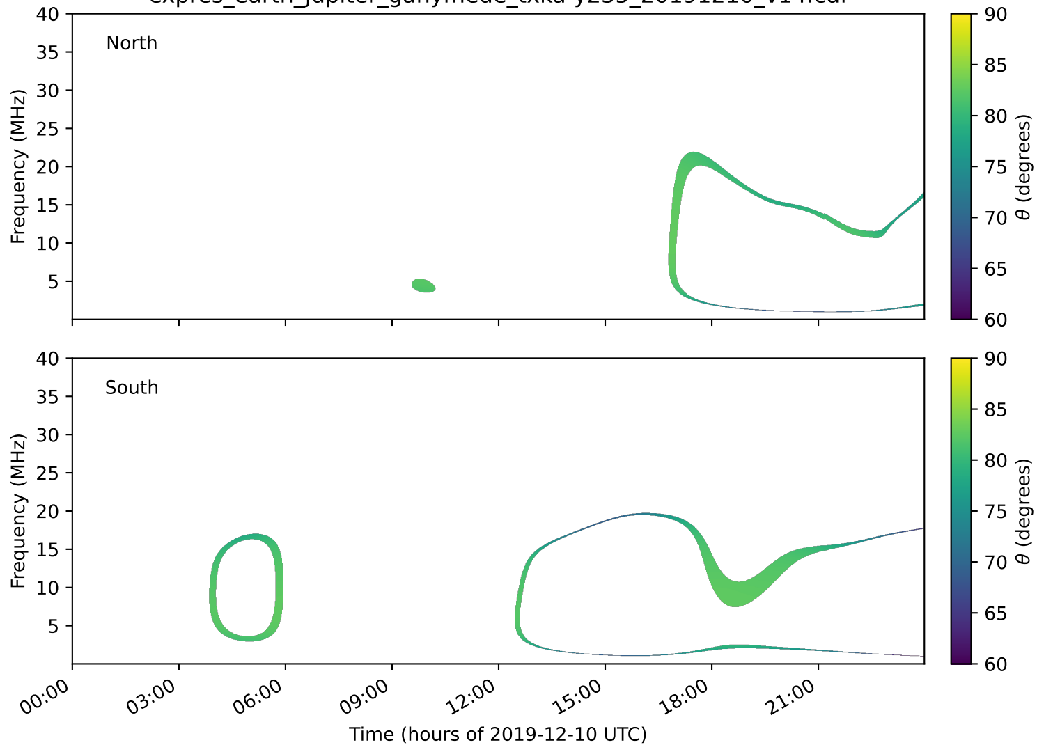
expres_earth_jupiter_ganymede_txka-y235_20191210_v14.cdf
