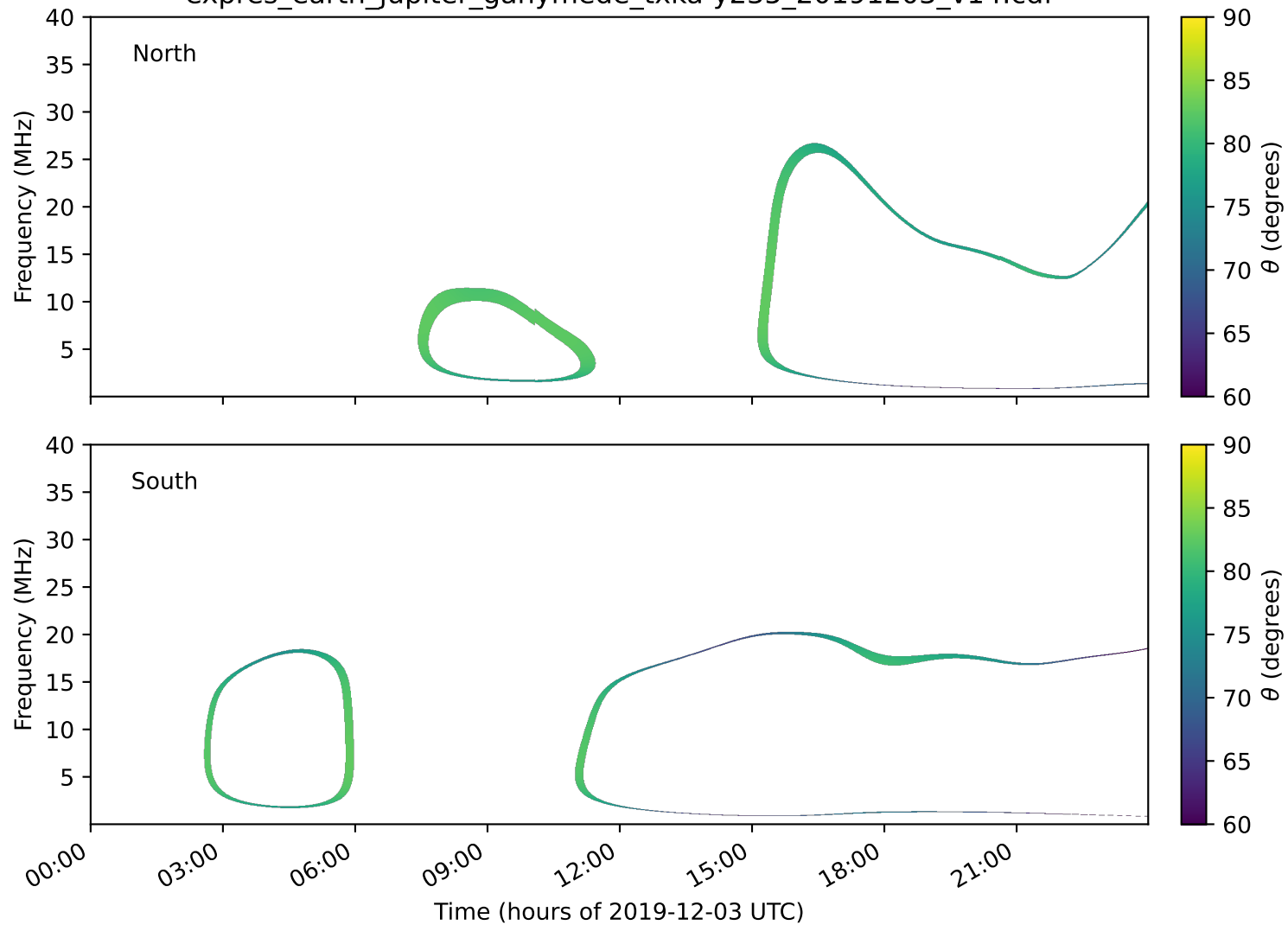
expres_earth_jupiter_ganymede_txka-y235_20191203_v14.cdf
