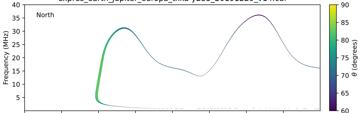
expres_earth_jupiter_europa_txka-y235_20191229_v14.cdf
