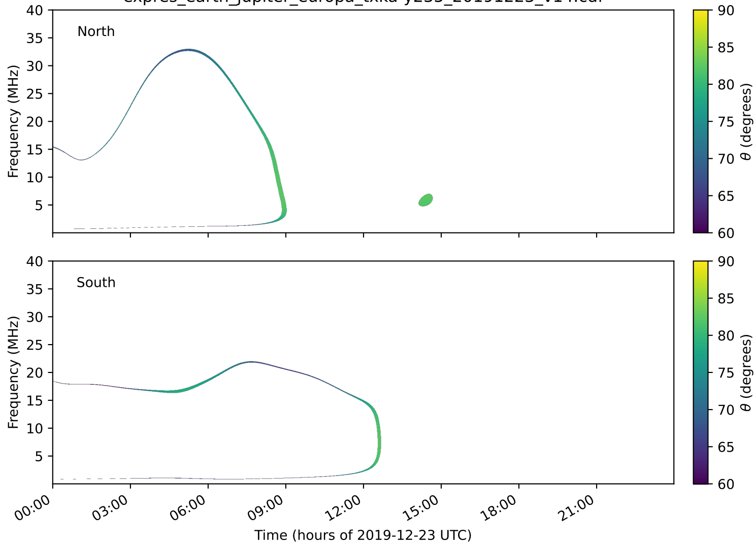
expres_earth_jupiter_europa_txka-y235_20191223_v14.cdf
