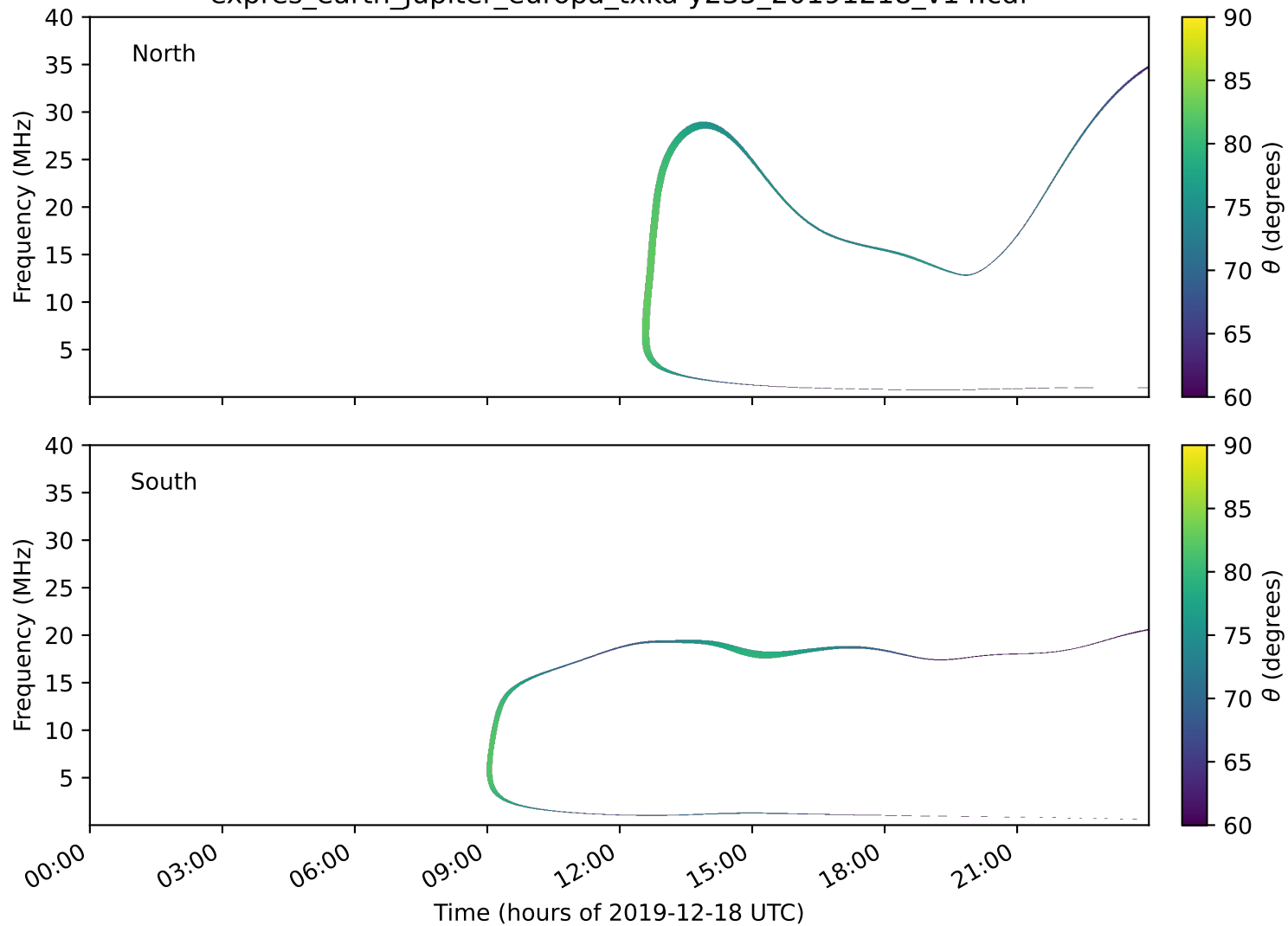
expres_earth_jupiter_europa_txka-y235_20191218_v14.cdf
