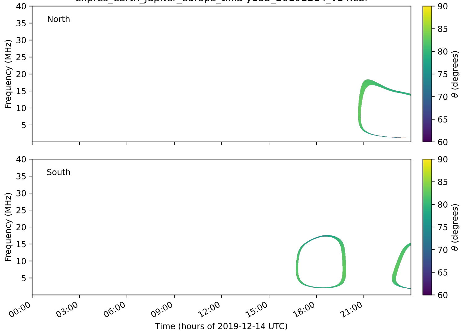
expres_earth_jupiter_europa_txka-y235_20191214_v14.cdf
