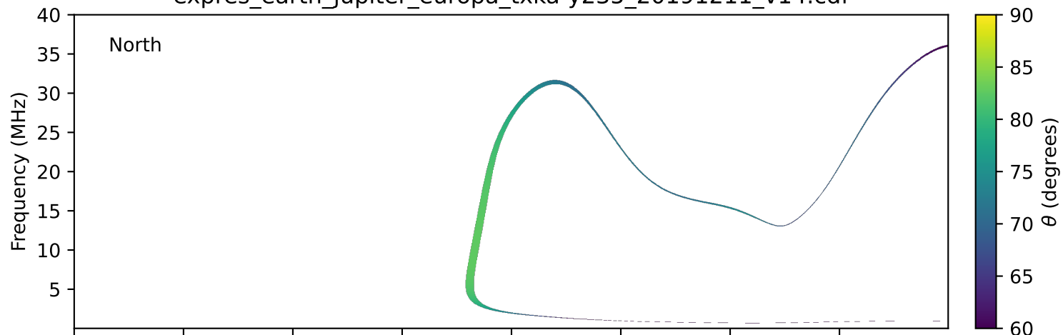
expres_earth_jupiter_europa_txka-y235_20191211_v14.cdf
