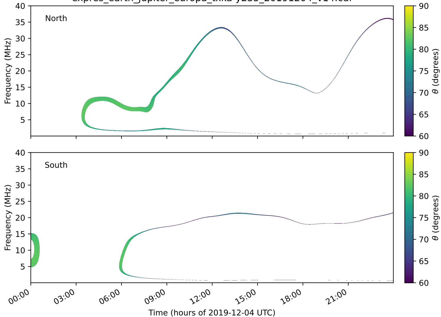
expres_earth_jupiter_europa_txka-y235_20191204_v14.cdf
