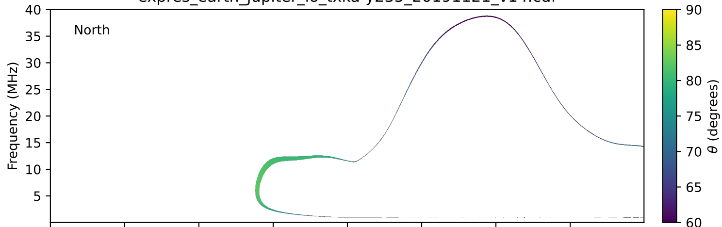
expres_earth_jupiter_io_txka-y235_20191121_v14.cdf
