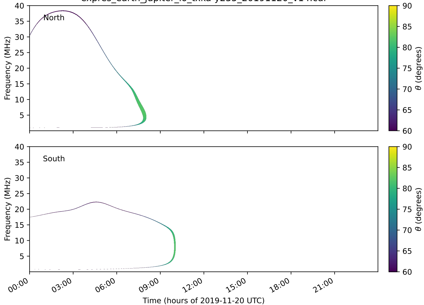
expres_earth_jupiter_io_txka-y235_20191120_v14.cdf
