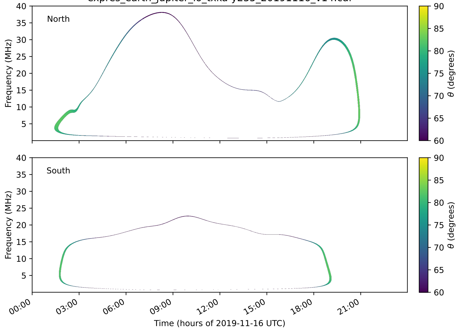
expres_earth_jupiter_io_txka-y235_20191116_v14.cdf
